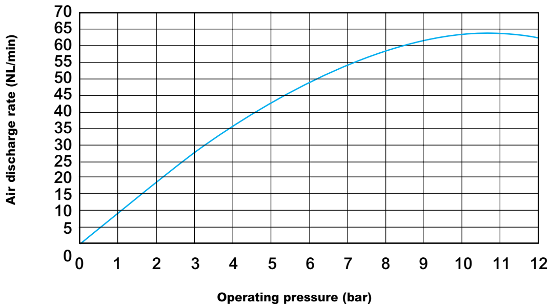
Air discharge rate - Operating pressure
